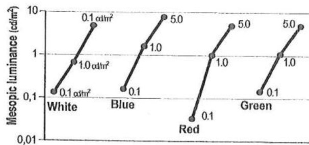
Figure 8 Calculated mesopic luminances of each luminance level organised by colour.
